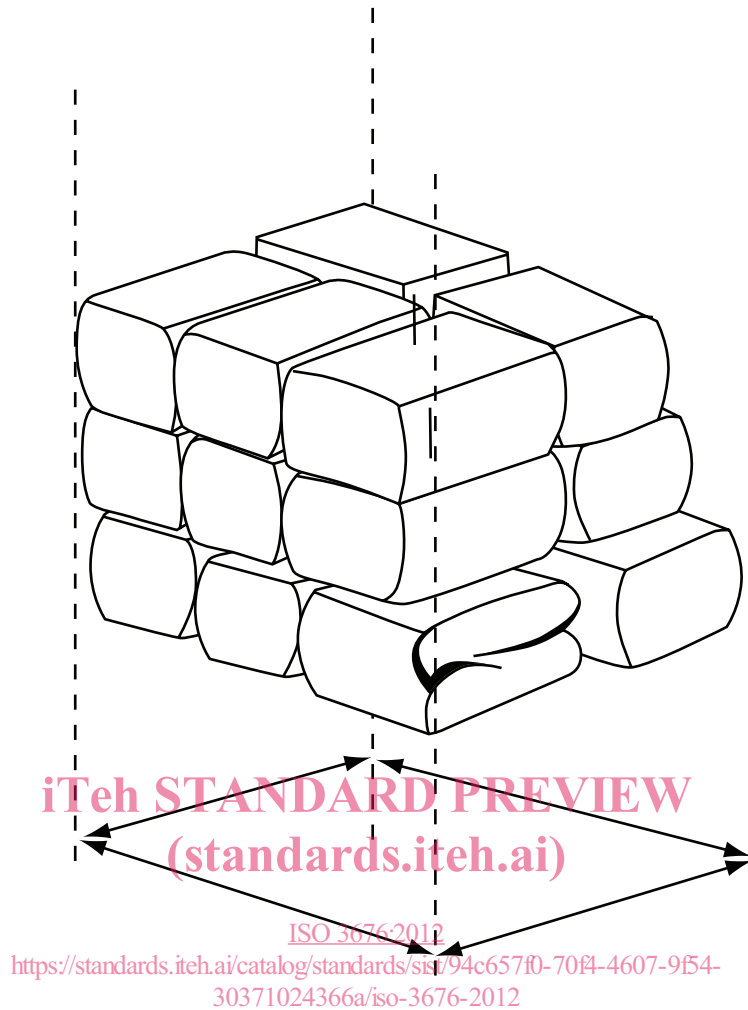
Figure 2 — Plan dimensions
