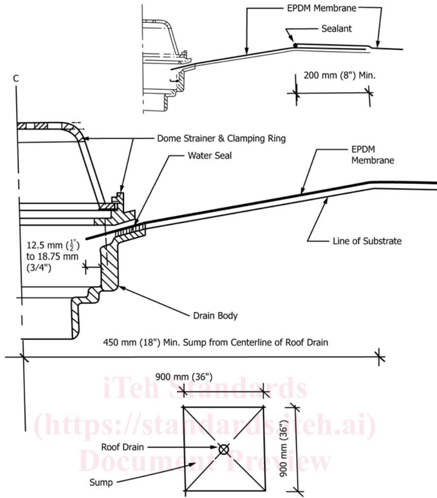
ASTM FIG. 4 Sump Transition
