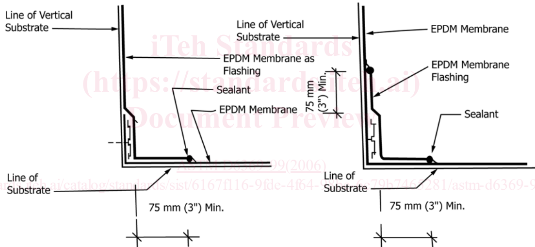
FIG. 2 Intersection of Horizontal and Vertical Planes
