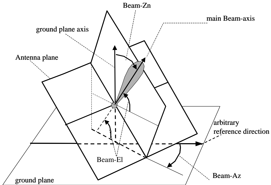
Figure 1b: Reference angles and planes for a passive (e.g. reflector) antenna iTeh STANDARD PREVIEW (standards.iteh.ai)
