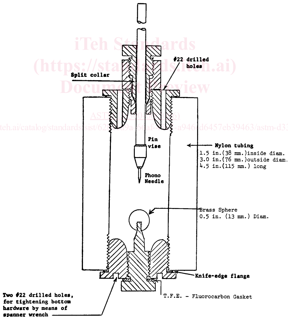
FIG. 1 Test Cell
