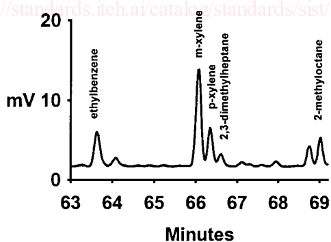
FIG. 7 p -xylene/2,3-dimethylheptane
