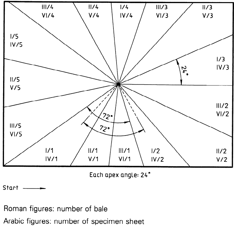
Figure 3 — Diagram illustrating how test pieces with constant angle at the apex are to be cut from specimen sheets selected according to the diagram given in figure 1
