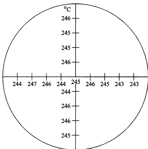
FIG. 2 Uniformity of Aluminum Plate Temperature at Set Temperature of 250°C
