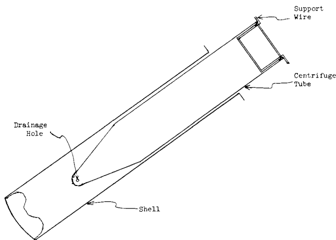
FIG. 1 Cross-section View of Centrifuge Tube Assembly
