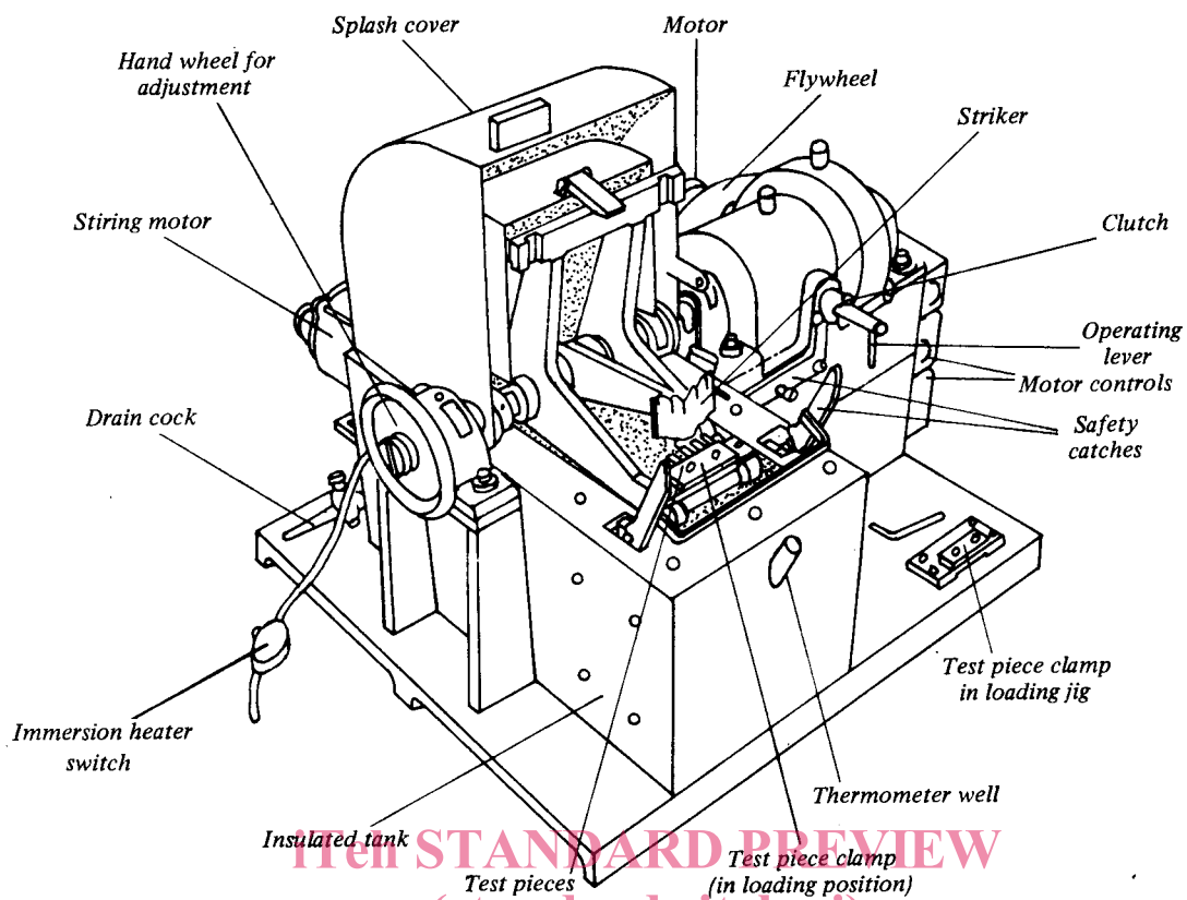
FIG. 3 - Motor-driven brittleness temperature tester
