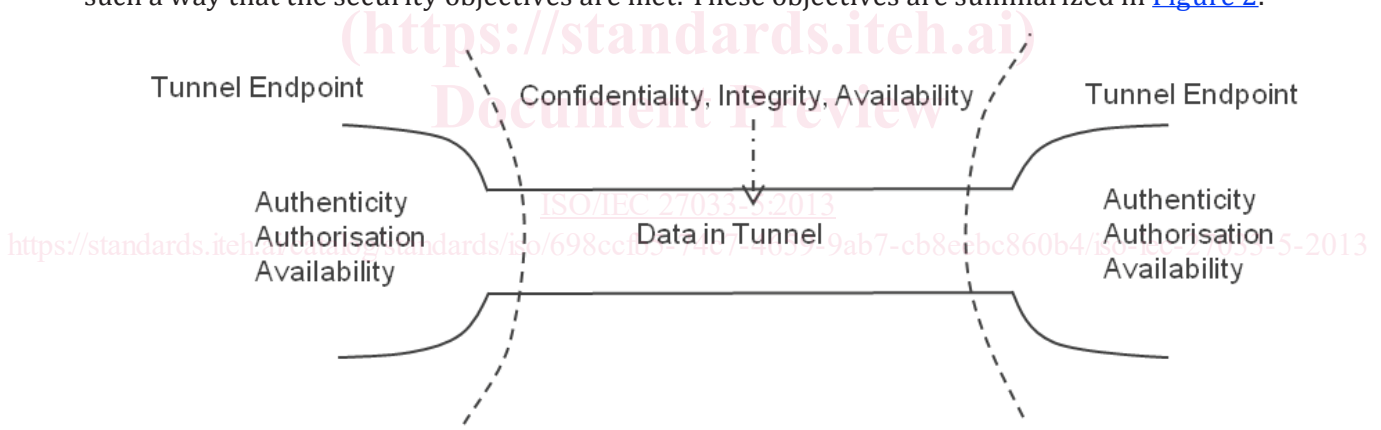
Figure 2 — Generic security requirements of VPNs mapped onto the underlying tunnel
