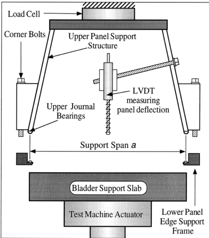
FIG. 2 Definition of Support Span for Specification of Panel Specimen Dimensional Tolerances
