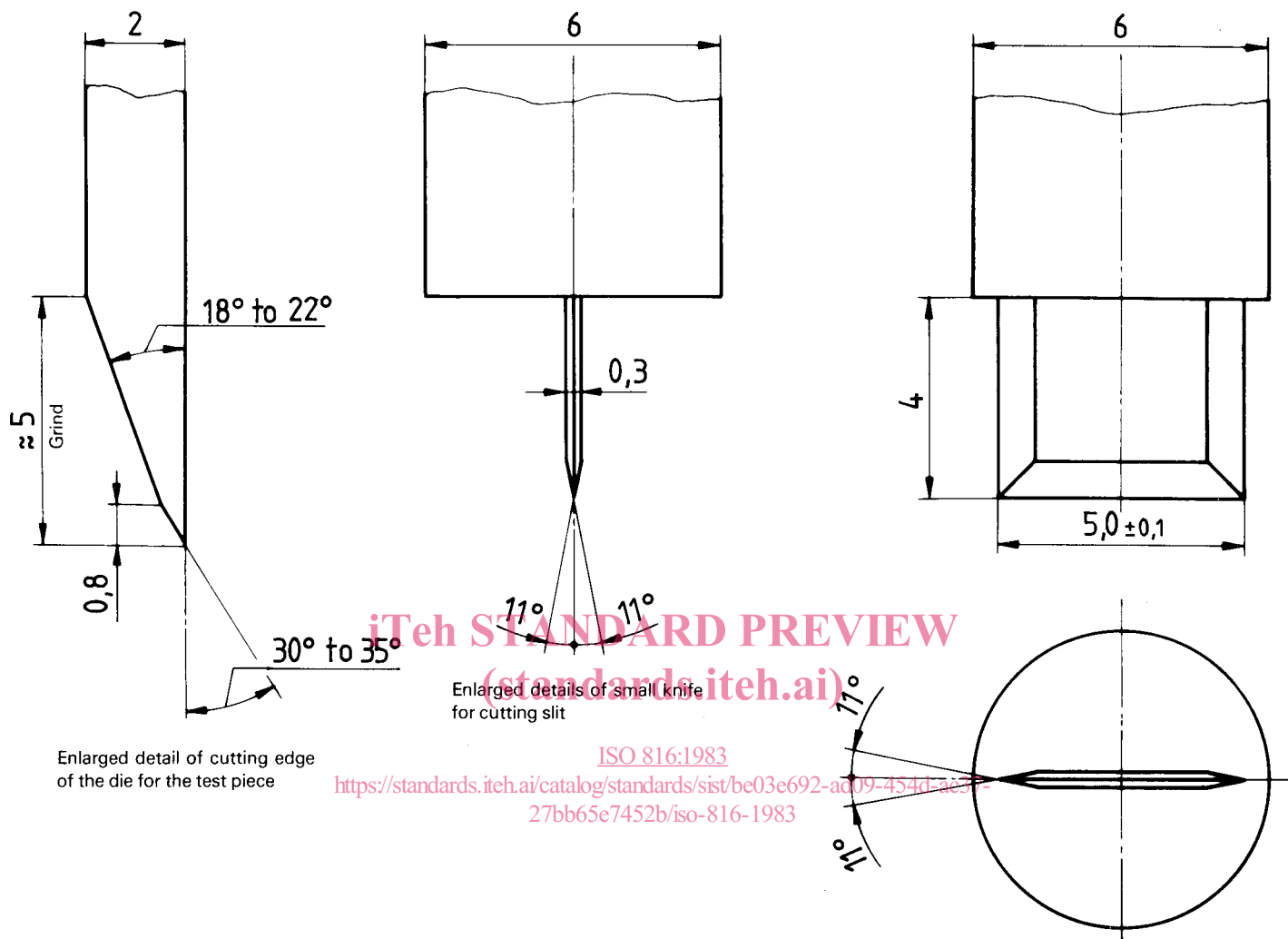
Figure 4 – Enlarged details of Delft tear test piece die cutting edges
