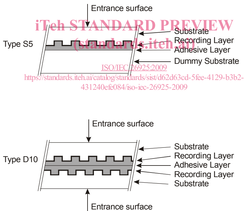
Figure 1 — Types of +RW HS disk
