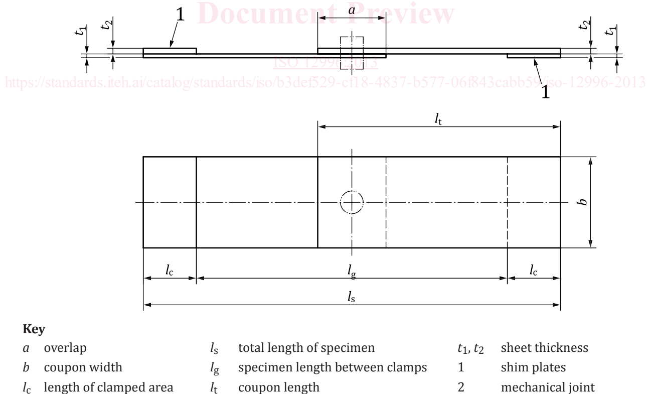
Figure 1 — Single-lap tensile shear test specimens
