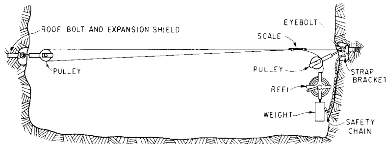
FIG. 3 Tape Extensometer with Vernier Readout and Deadweight
