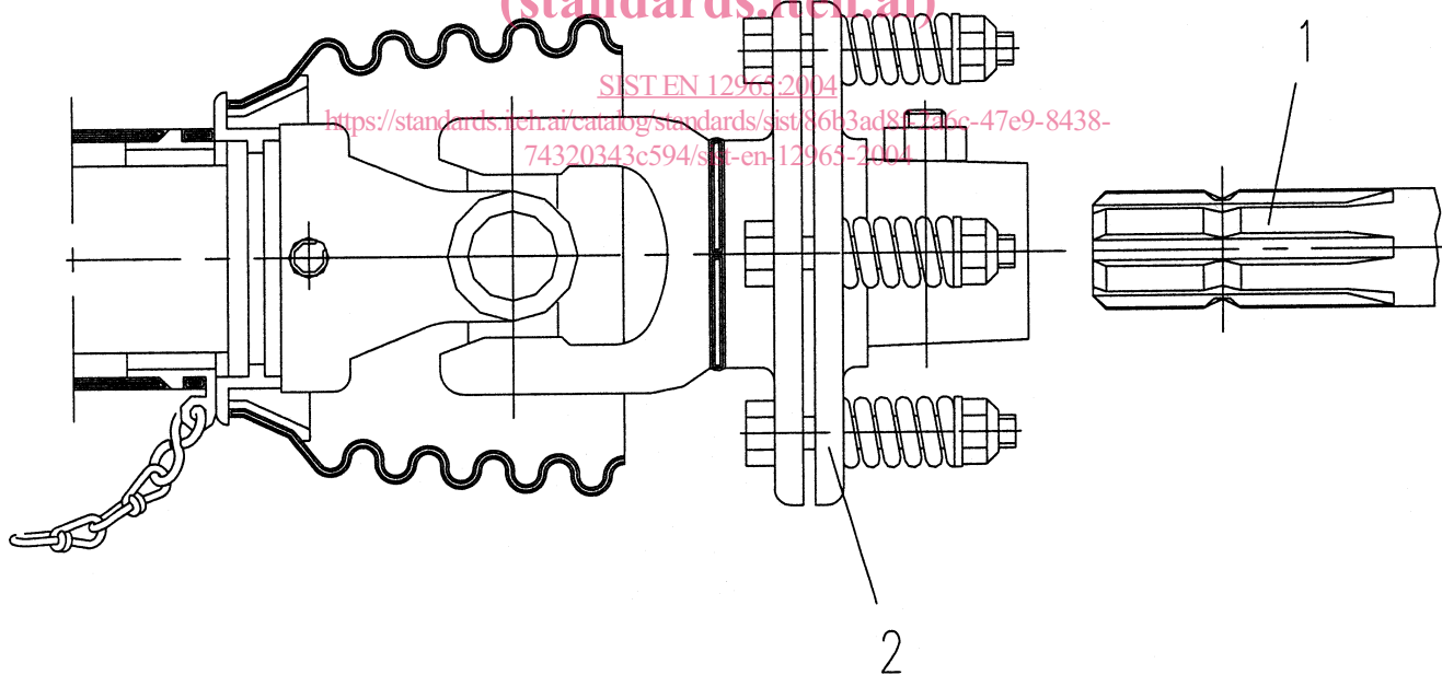
Figure 2 — Example of overrun device iTeh STANDARD PREVIEW (standards.iteh.ai)
