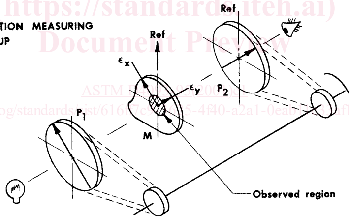
FIG. 5 Direction Measuring Set-up
