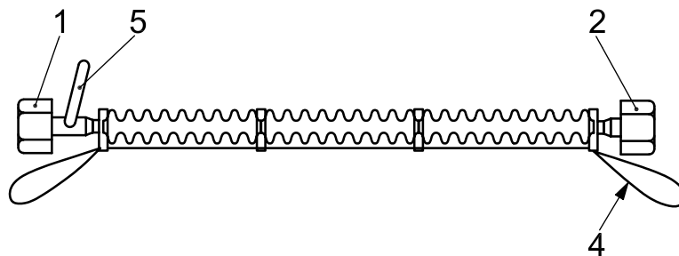
c) Corrugated metal (e.g. stainless steel) hose fitted with retaining straps
