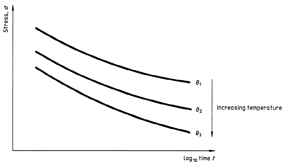
Figure 5 — Creep-to-rupture curves
