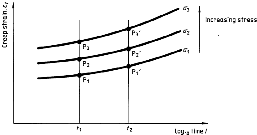
Figure 2 — Creep curves
