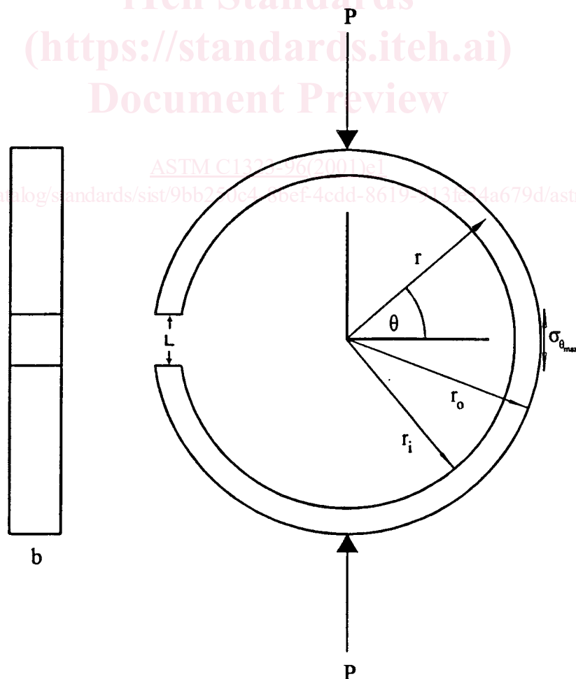
FIG. 1 C-Ring Test Geometry with Defining Geometry and Reference Angle (θ) for the Point of Fracture Initiation on the Circumference
