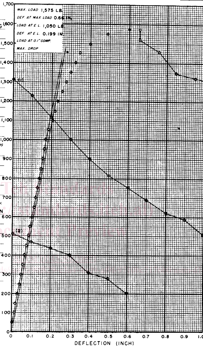
FIG. 5 Sample Data Sheet for Static Bending Test
