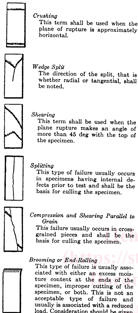
FIG. 10 Types of Failures in Compression
