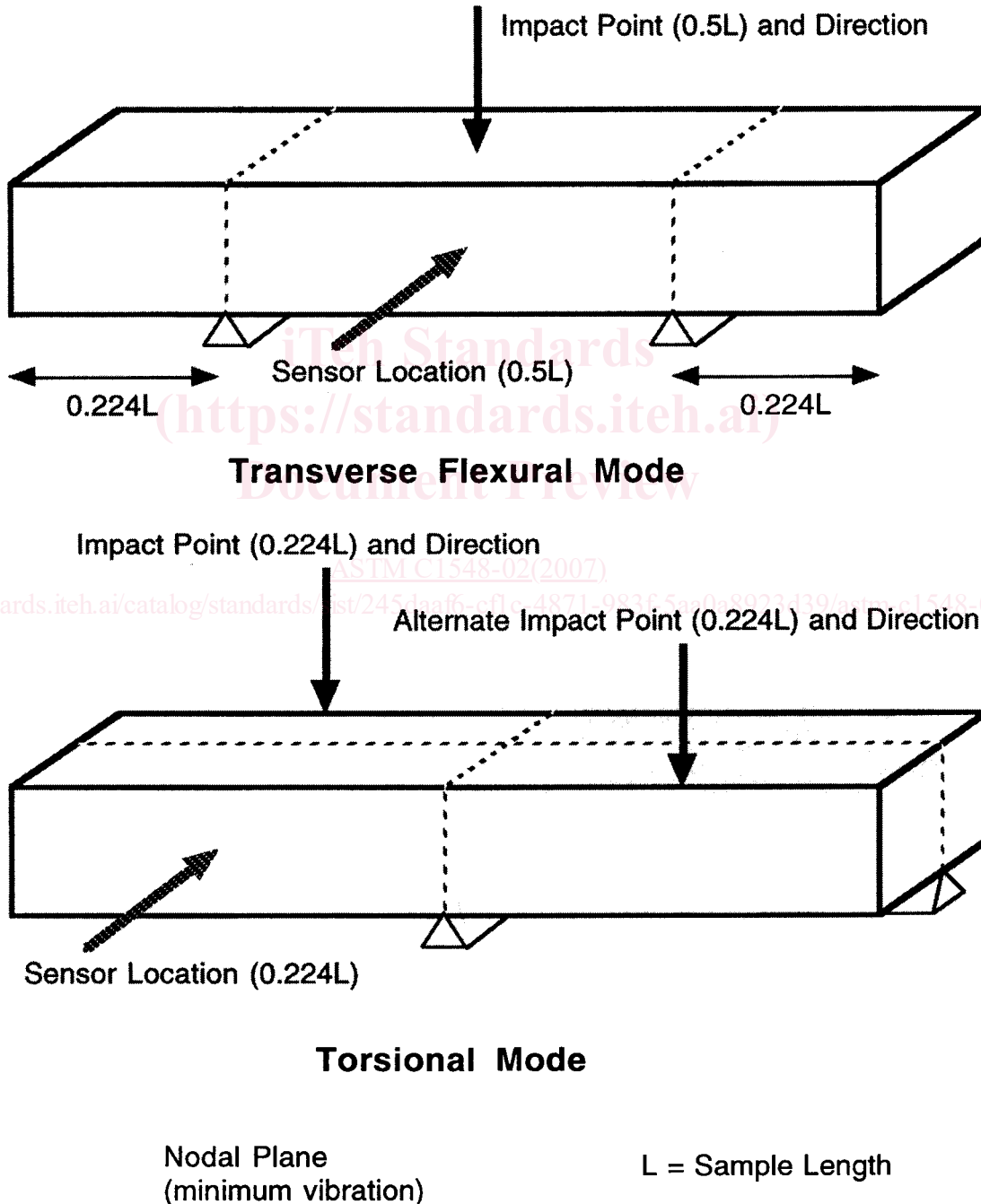
FIG. 2 Impact Points and Transducer Locations
