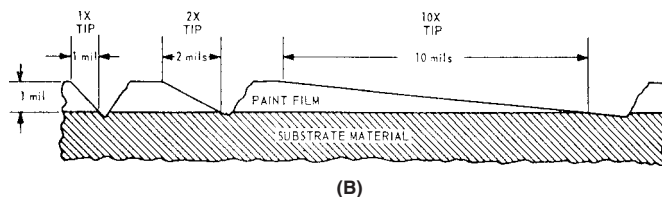
FIG. 2 Grooves Made by 1×, 2×, and 10× Cutting Tips (continued)
