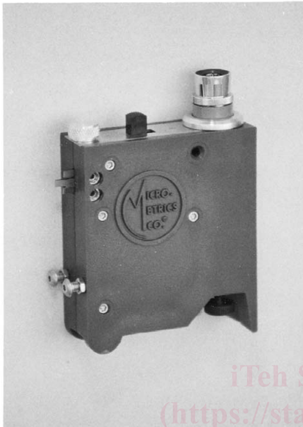
FIG. 1 Tooke Inspection Gage 3
