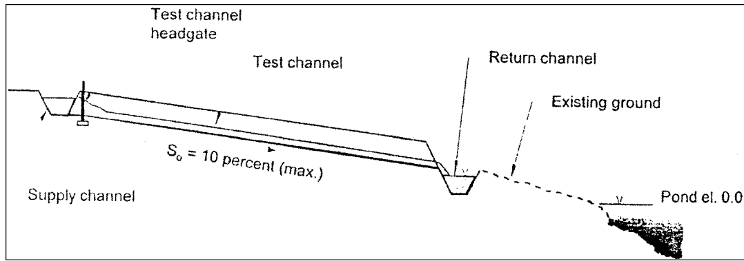
FIG. 2 Typical Channel Profile
