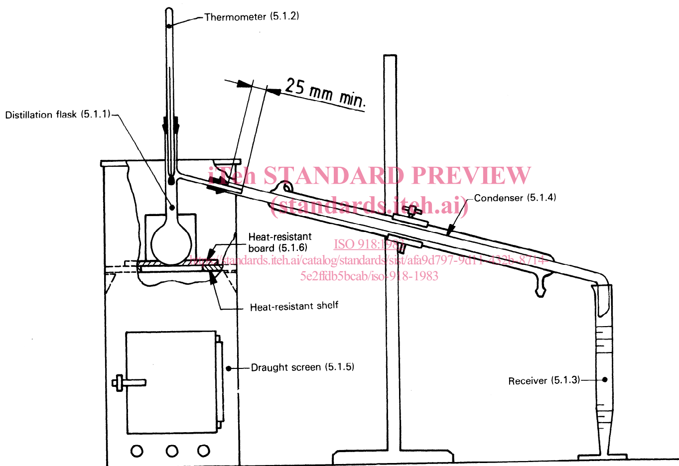
Figure 1 – Assembly of distillation apparatus (5.1)
