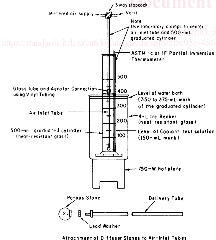
FIG. 1 Schematic Drawing of Apparatus for Glassware Foam Test
