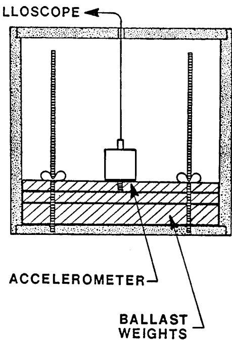
FIG. 2 Test Block
