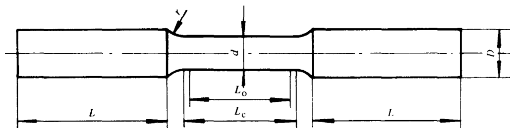
FIGURE – Tensile test bar
