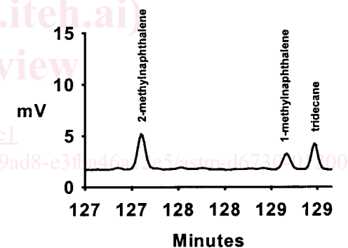
FIG. 9 1-methylnaphthalene/tridecane
