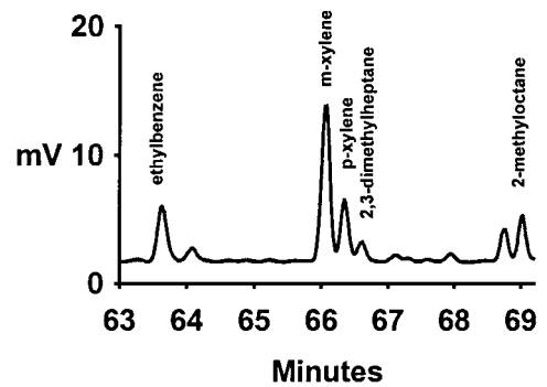
FIG. 7 p -xylene/2,3-dimethylheptane
