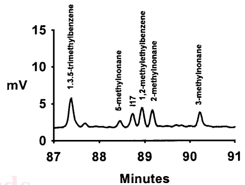
FIG. 8 I17 (unknown)/1,2-methylethylbenzene
