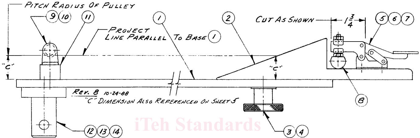
FIG. 1 Overall Fixture
