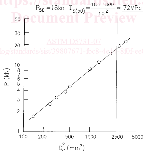
FIG. 6 Procedure for Graphical Determination of I_{s(50)} from a Set of Results at D_e Values Other Than 50 mm 6
