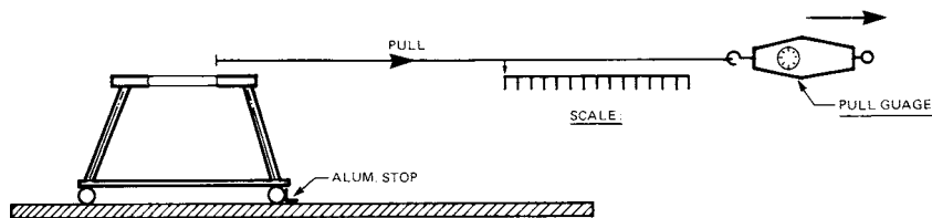
FIG. 6 Tip Resistance Setup
