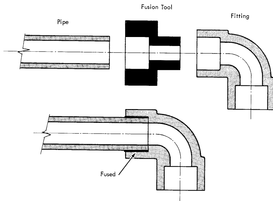
FIG. 1 Socket Fusion
