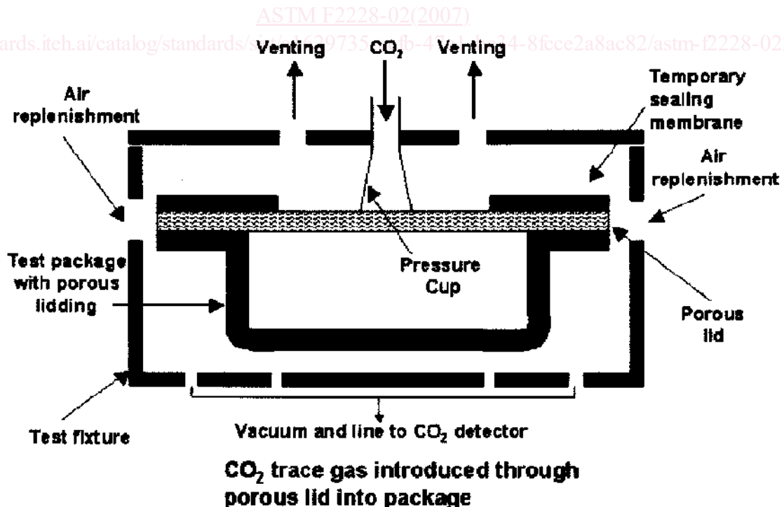
FIG. 1 Schematic of Test Fixture and Test Package
