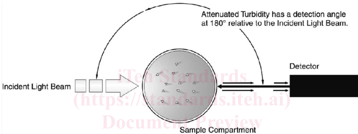
FIG. 5 Geometric Design of an Attenuated Measurement
