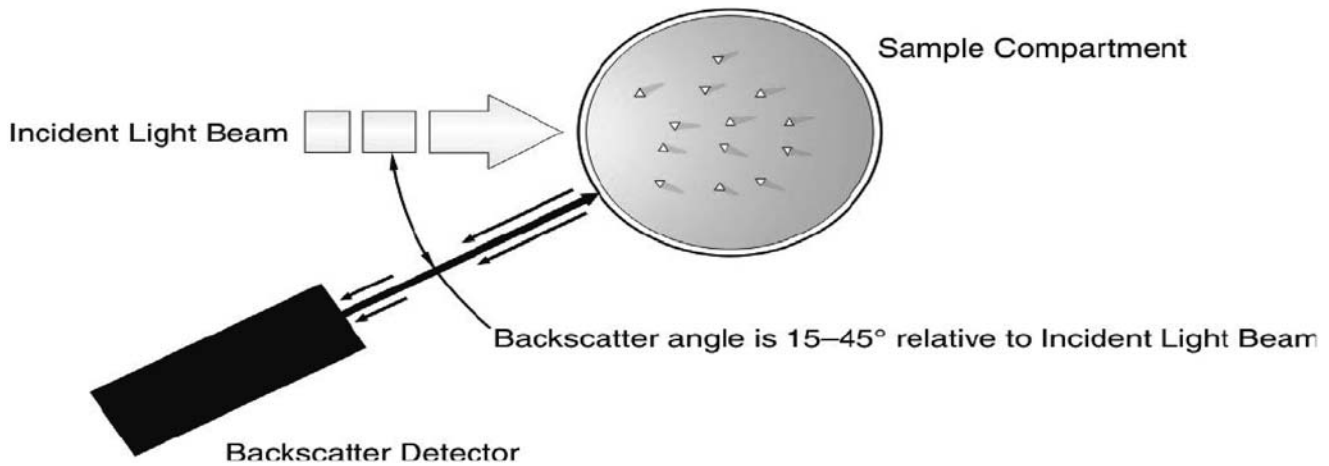
FIG. 4 Geometric Diagram of a Backscatter Measurement
