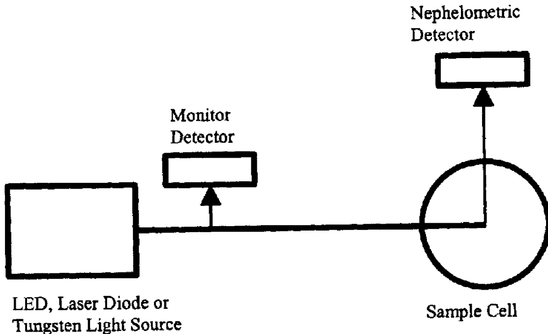
FIG. 1 Typical Nephelometer
