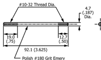
NOTE 1—All dimensions are in millimetres (inches). FIG. 4 Holding Rod
