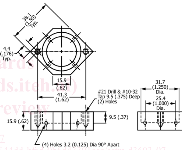
NOTE 1—All dimensions are in millimetres (inches). FIG. 3 Specimen Holder
