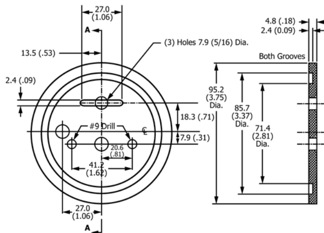
NOTE 1—All dimensions are in millimetres (inches). FIG. 2 Beaker Cover
