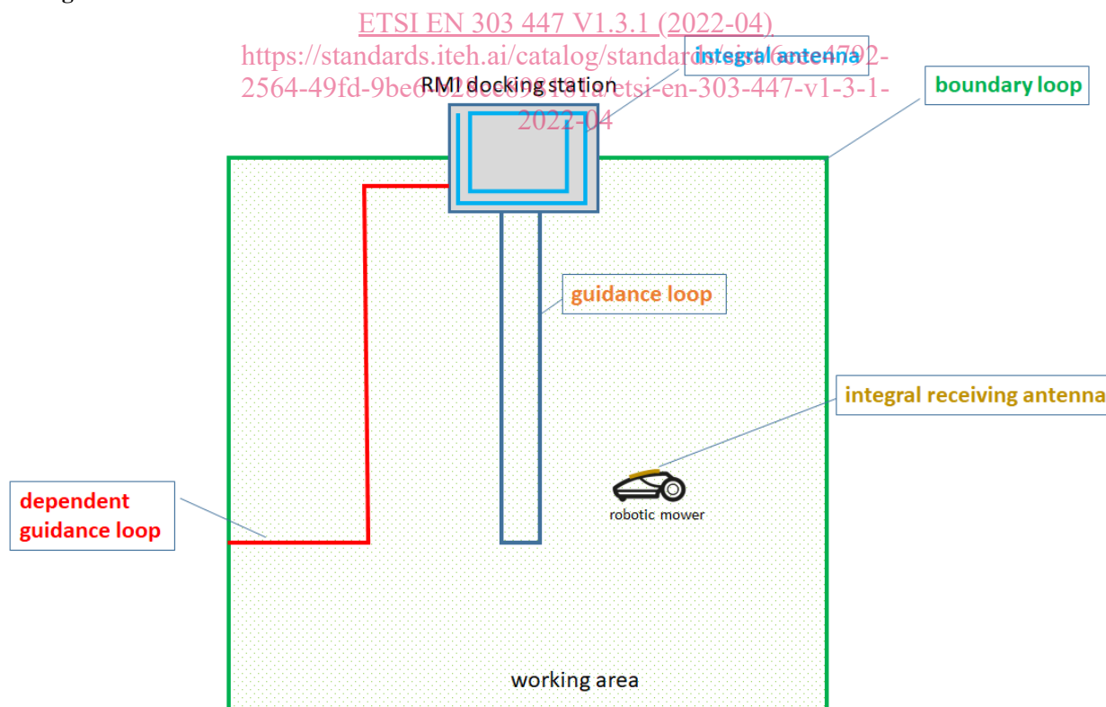
Figure 2: Overview of an RMI system, including the different possible antenna/loops
