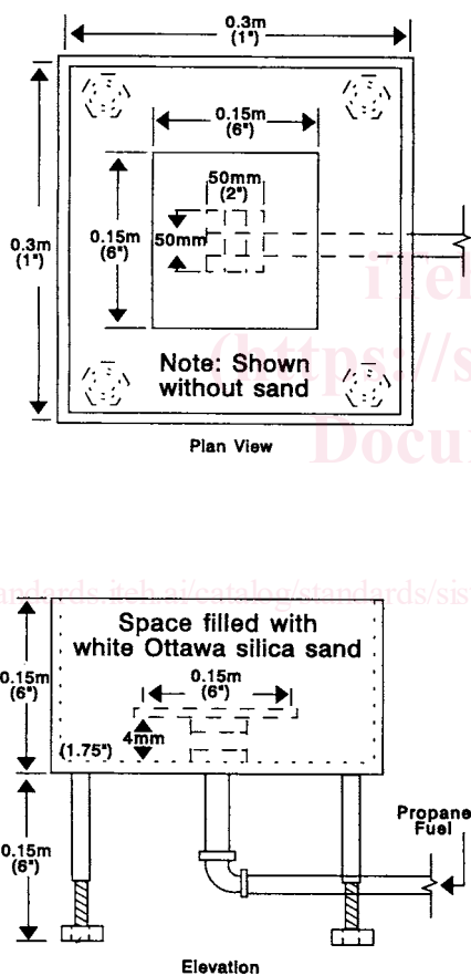
NOTE 1—See text for tolerances. FIG. 9 Calibration Gas Burner
