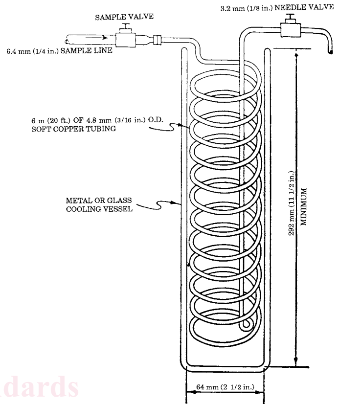
FIG. 2 Precooling Equipment
