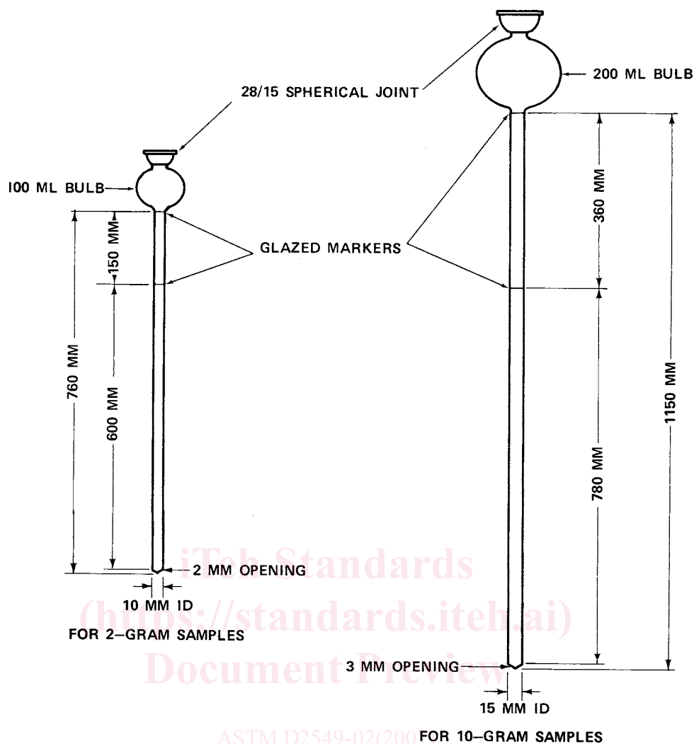
ASTM D2549-02(2007) FOR 10-GRAM SAMPLES FIG. 1 Chromatographic Columns
