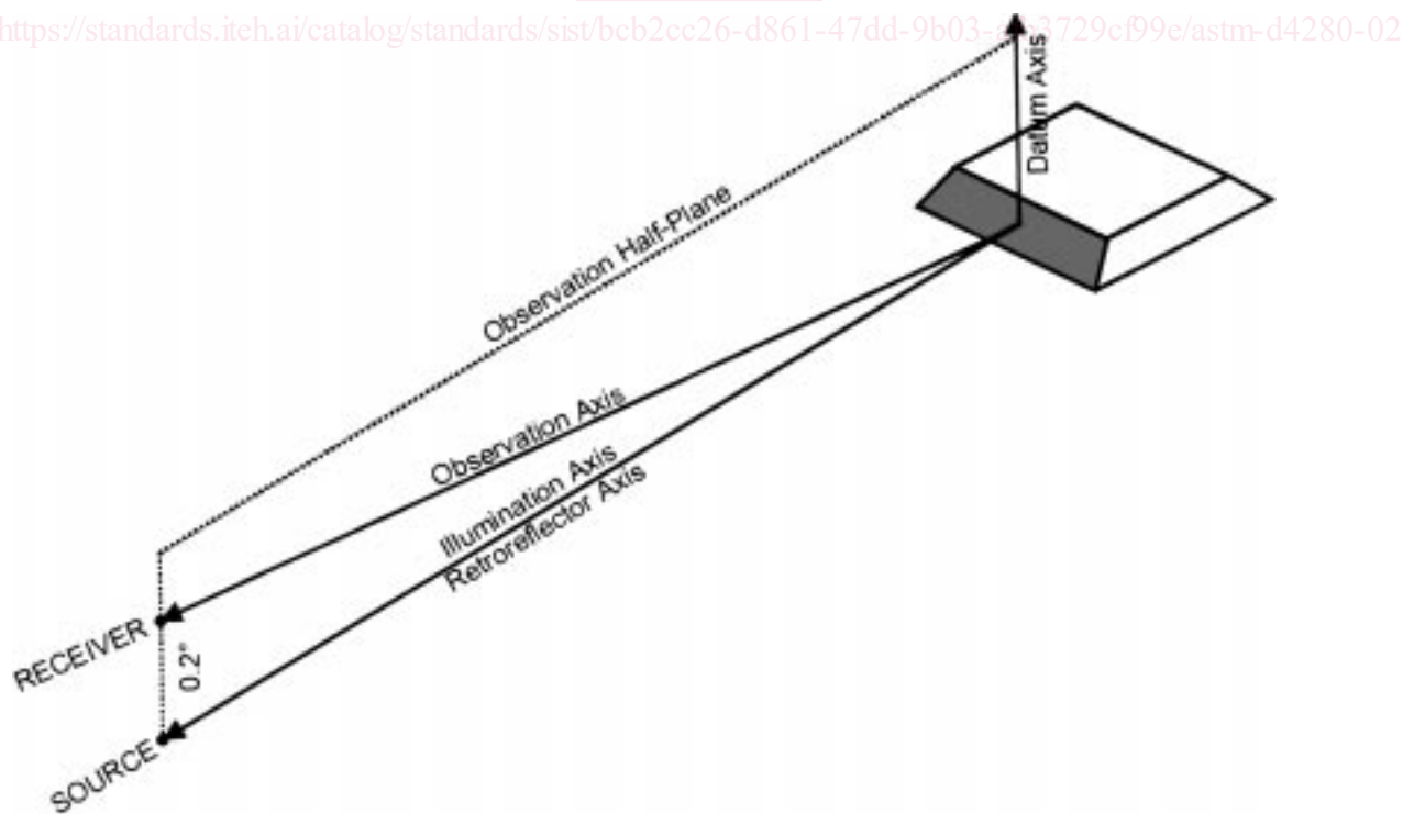
FIG. 2 Position of Marker for Photometry, 0^\circ Entrance Angle
