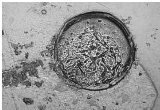
FIG. X1.1 Digital Photograph of Acid Etch Produced During Field Exposure (Jacksonville, FL, 50 x magnification)
