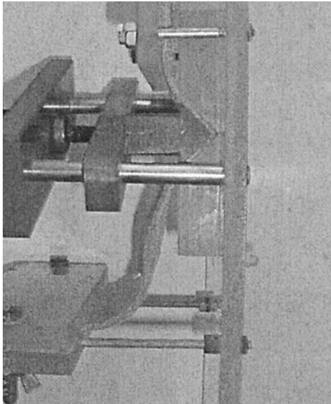
FIG. 1 Crimping Wedge
