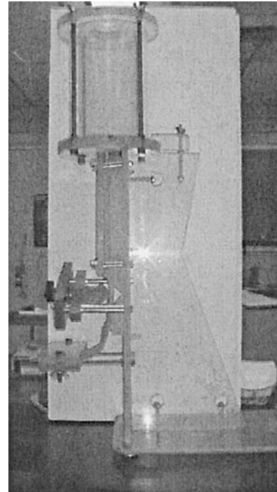
FIG. 2 Complete Crimp Test Apparatus
