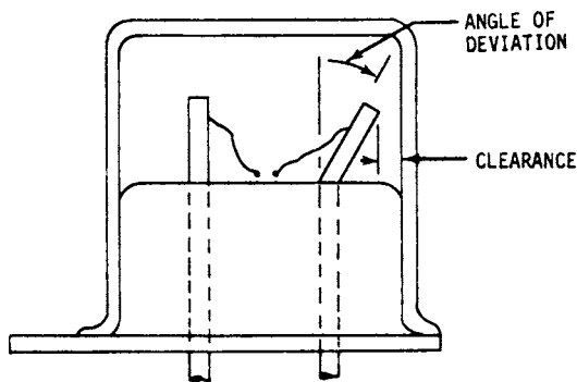
FIG. 3 Transistor—Post-Position Irregularities
