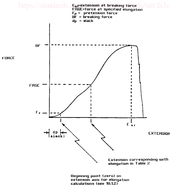
FIG. 1 Force-Extension Curve
