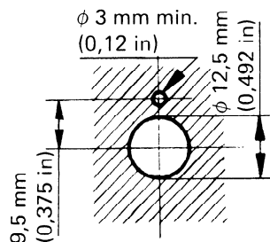
FIGURE 2 – Panel drilling
