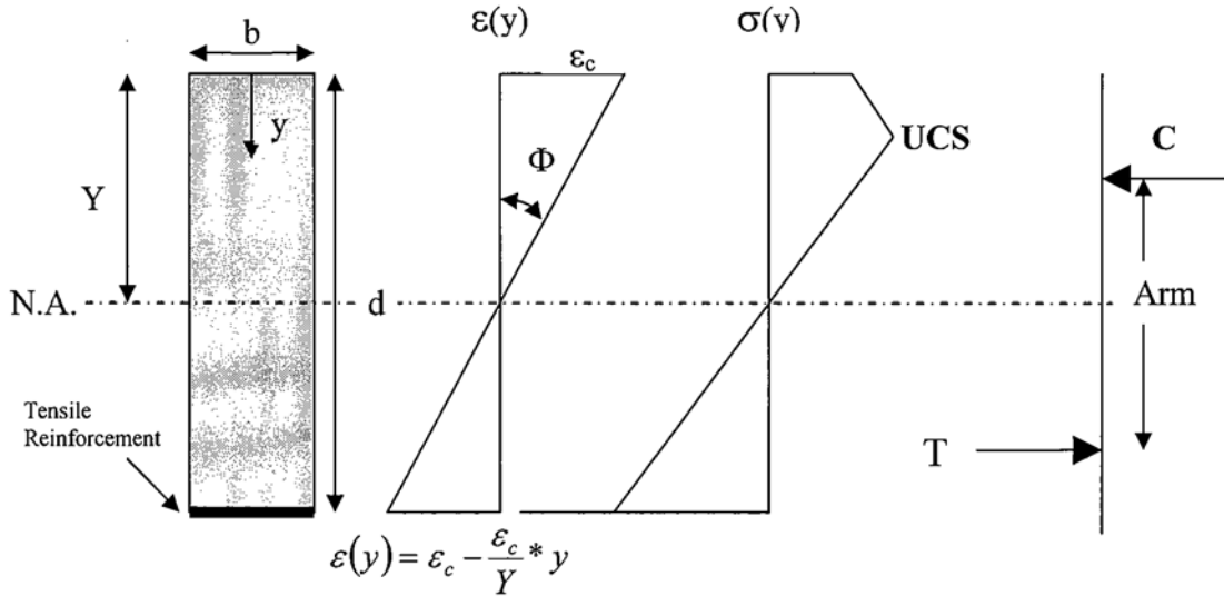
NOTE 1—A simplified rectangular block stress distribution can be used but it must be shown that it accurately represents the stress distribution. FIG. 2 Example of Beam Section with Strain, Stress, and Force Diagrams
