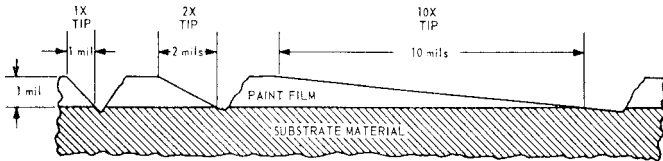
FIG. 2 Grooves Made by 1x, 2x, and 10x Cutting Tips
