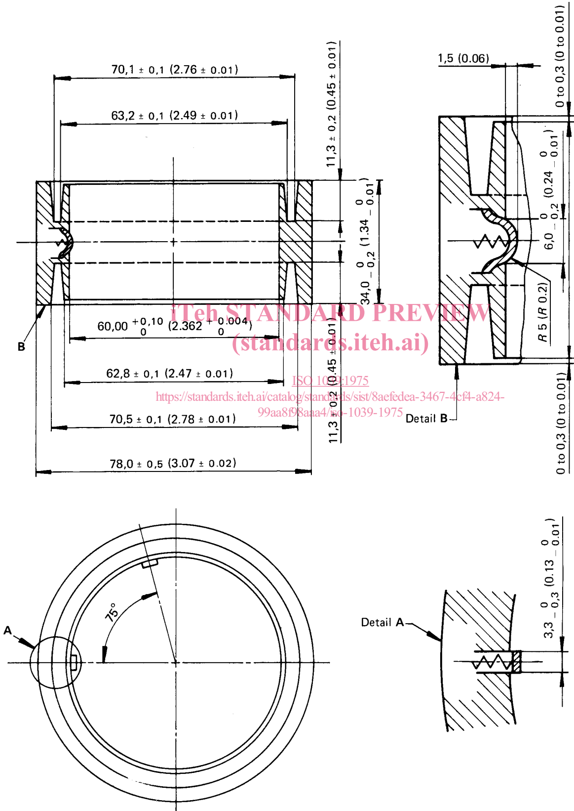
FIGURE 3 – Dimensions for core with light lock groove
