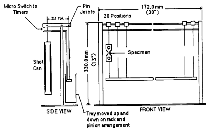
NOTE 1—The number of positions in the test frame is optional. FIG. 2 Constant Stress Loading Apparatus Consisting of Twenty Specimen Test Positions
